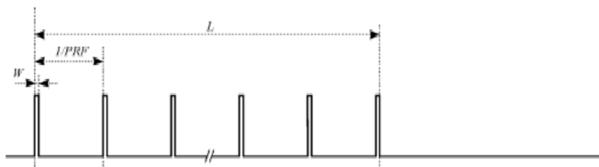
Figure 1: General structure of a single burst DFS test transmission
